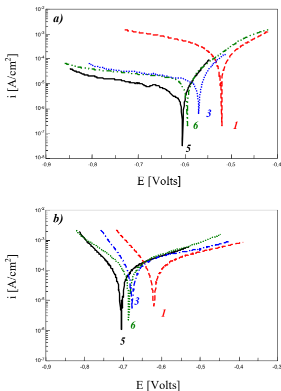
Fig. 2. Polarisation curves of the alloys No. 1, 3, 5 and 6 after: a) 1 hour, b) 168 hours of exposure in 3% aqueous NaCl solution
