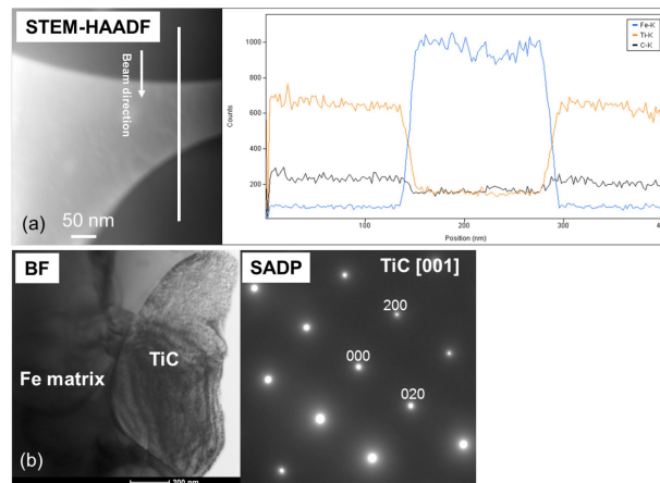
Fig. 5. STEM-HAADF image and result of line scan analyze (a) and BF image and corresponding SADP image (b) of interfaces in TiC-Fe MMCs.
