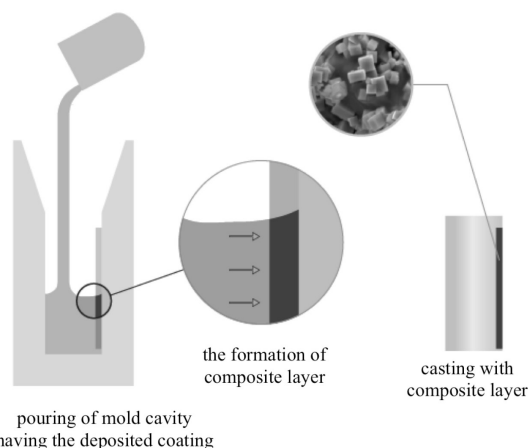
Fig. 1. Schematic presentation of the formation of the composite layer 1D in situ in the casting
