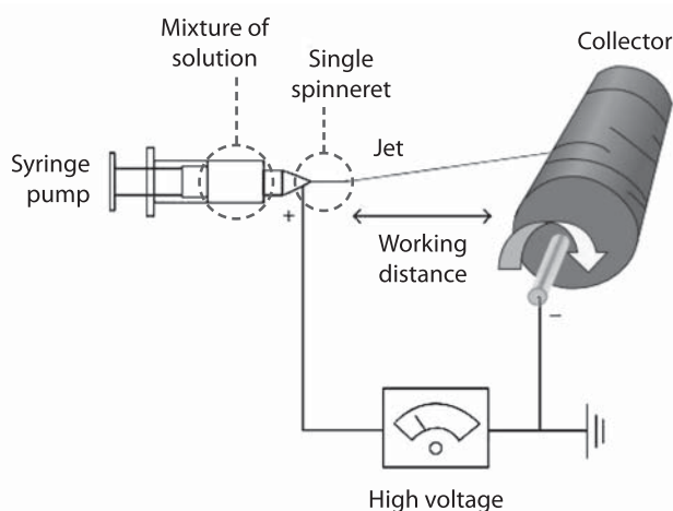
Fig. 1. Schematic diagram of the electrospinning setup (Mori et al. 2015)
