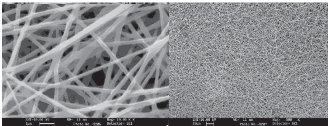
Fig. 2. Scanning electron microscope (SEM) photographs of the diameter distribution of the electrospun nanofibers of the different formulations
