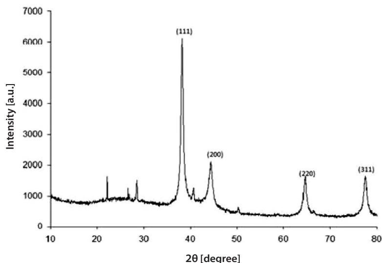
Fig. 2. X-ray diffraction (XRD) spectrum of silver nanoparticles (Ag NPs) extracted from Trichodesma indicum
