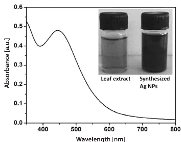
Fig. 1. Shows UV-vis spectra formation of the Ag NPs from leaf extract of Trichodesma indicum . Spectrum of Ag NPs formed due to addition of T. indicum leaf extract to silver nitrate solution
