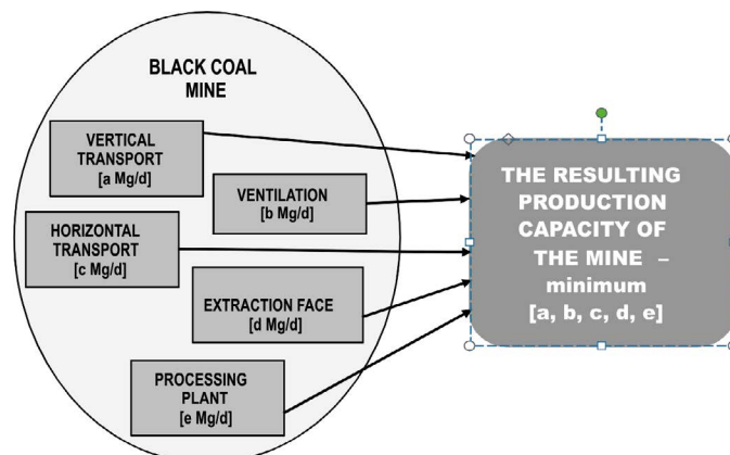
Fig. 2. The main elements of a production process determining the production capacity of a black coal mine Source: own research
