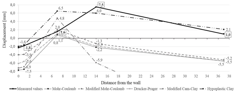
Fig. 11. Vertical displacements of terrain – construction stage 9
