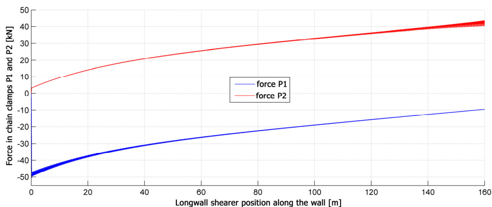
Fig. 7. Change in the value of P_1 and P_2 forces when the longwall shearer pass through the wall
