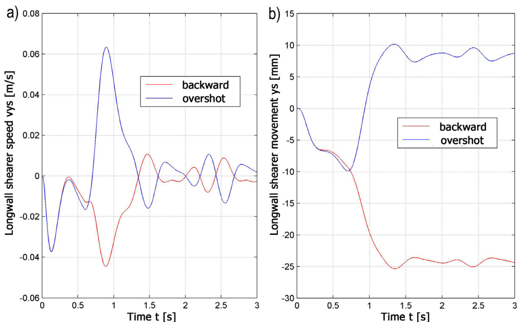
Fig. 9. Effects of unit direction of rotation on speed v_{ys} and displacement y_s
