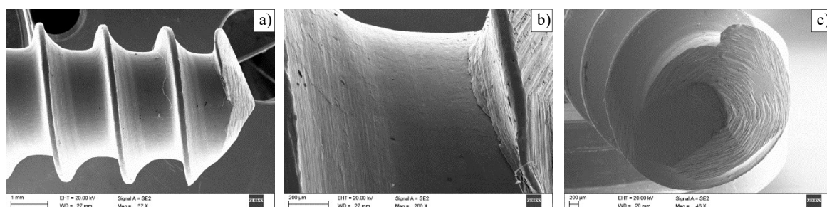
Fig. 4. Results of SEM test for Group II bone screws: a) thread contour is regular, visible minor damage, mag. 37×, b) the surface of the screw with a small number of calcium molecules, mag. 200×, c) Visible considerable wear of screw front surface, mag. 46×
