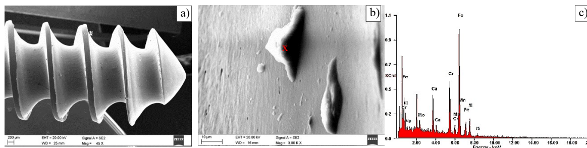
Fig. 3. Results of SEM test for Group I bone screws: a) irregular thread contour and mechanical damage to the surface of the screw, mag. 45×, b) a single molecule of calcium, the residue of bone of the patient, mag. 3000×, c) EDS spectrum of the elemental composition
