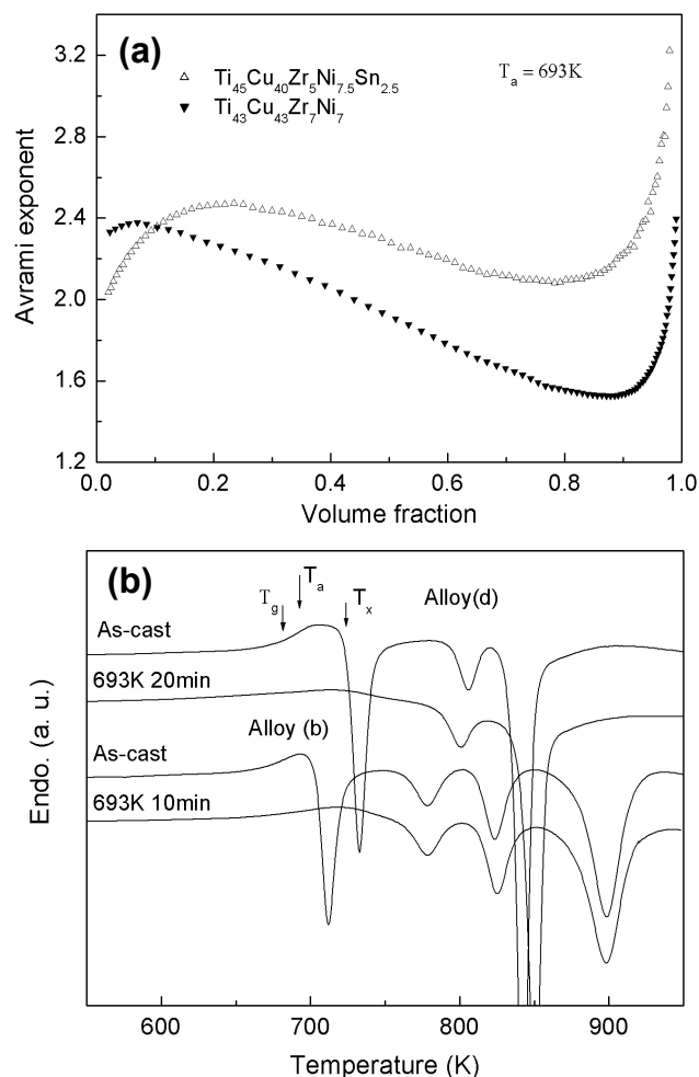
Fig. 4. (a) Avrami exponents of alloy (b) and (d) changing with volume fraction of crystallites upon 693K isothermal annealing, and (b) DSC scans of isothermal annealed samples of alloy (b) and alloy (d) compared with as-cast samples
