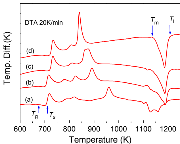
Fig. 1. DTA scans for the alloys from (a) to (d) listed in Table 1 at a heating rate of 20 K/min
