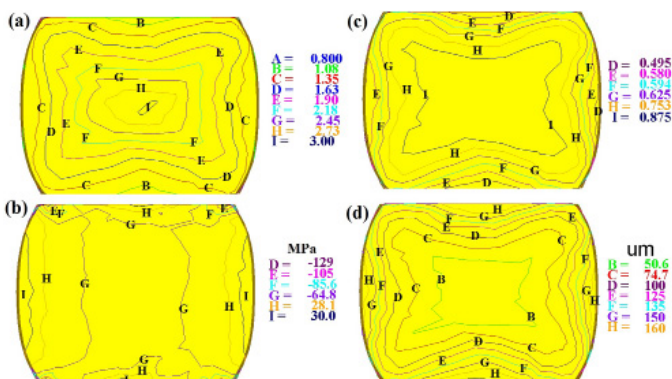
Fig. 11. Distribution of effective strain (a), mean stress (b), the dynamically recrystallized volume fraction (c) and mean grain size (d) on the cross-section of the specimen X6CrNiTi18-10 steel during the cogging process in flat anvils after the eighth pass (forging ratio of 2.25)
