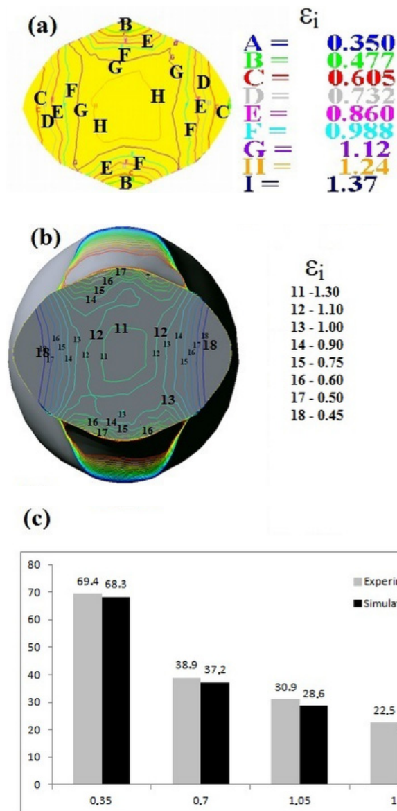
Fig. 14. Comparisons of the theoretical (a) and experimental (b) effective strain ( \epsilon_1 ) distribution on the cross-sectional surfaces of X6CrNiTi18-10 steel specimens deformed in radial-rhombic anvils with an impression angle of \alpha = 135^\circ \times 135^\circ (relative feed l_w = 0.75 ; true strain \epsilon_1 = 0.70 ), (c) comparisons between the experimental and simulated results (average grain sizes in the centre of the specimens deformed in radial-rhombic anvils at different true strain)
