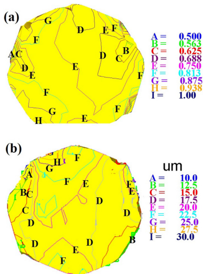
Fig. 10. Distribution of the dynamically recrystallized volume fraction (a) and mean grain size (b) on the cross-section of the specimens X6CrNiTi18-10 steel during the cogging process in radial-rhombic anvils with an impression angle of \alpha = 135^\circ \times 135^\circ after fourth pass
