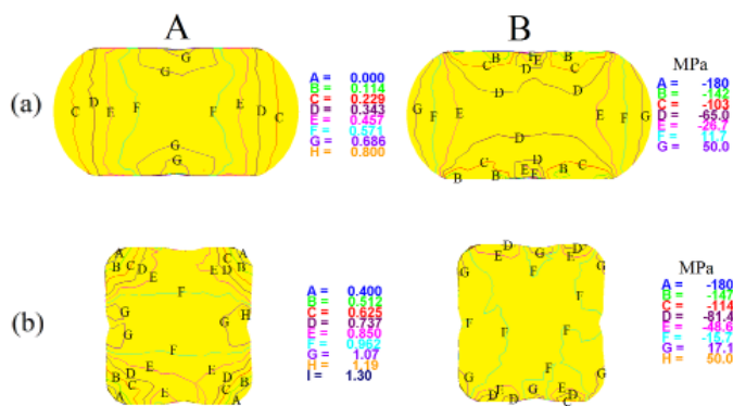
Fig. 6. Distribution of effective strain (A) and mean stress (B) on the cross-section of the specimens X6CrNiTi18-10 steel during the cogging process in angular convex anvils with an angle of 135^\circ after the first reduction (a) and the second reduction (b). True strain \varepsilon_h = 0.35
