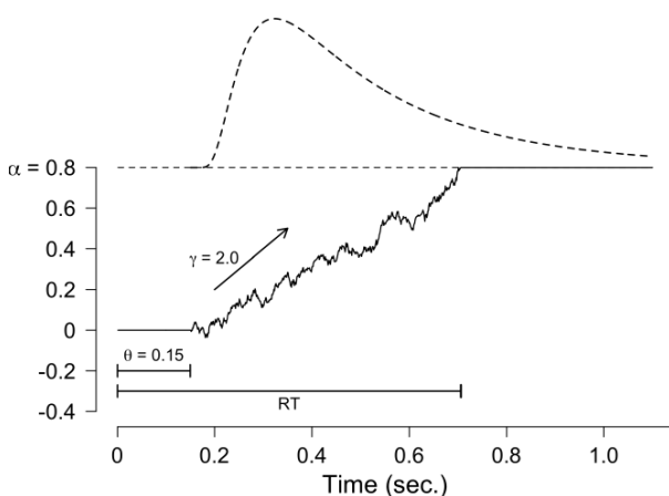
Figure 3. The shifted Wald as a cognitive model, describing RT as the time for an accumulator to drift toward and hit a single boundary of height 0.8 at a drift rate of 2.0. The nondecision time 0.15 represents the component of RT which is not due to this accumulation process. The solid black line represents the accumulator for a single trial, whereas the dashed upper curve represents the shifted Wald distribution formed by collecting RTs for many such trials.
