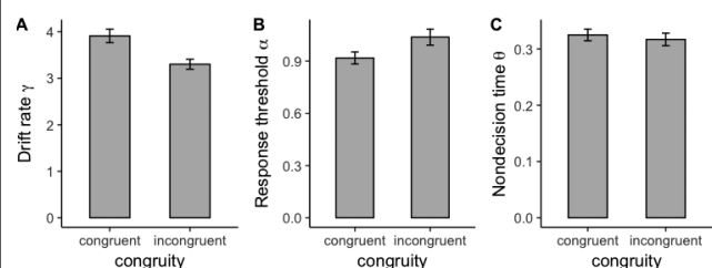
Figure 5. Means of shifted Wald parameters presented as a function of congruity (congruent versus incongruent). Panel A depicts drift rate, which indexes rate of information accumulation from stimuli. Panel B depicts response threshold, which indexes the amount of accumulated information required before response initiation. Panel C depicts nondecision time, which indexes the amount of time required for nondecision processes (e.g., encoding and response generation).
