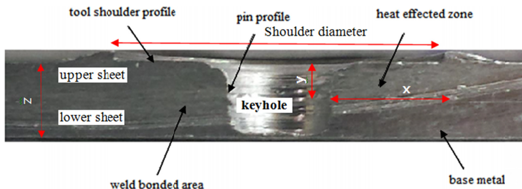
Fig. 7. Schematic illustration of the cross section of friction stir spot weld. x : stir zone thickness, y : the thickness of the upper sheet and z : total materials thickness
