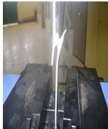
Fig. 11. Shear specimen during the tensile test
