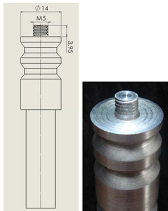
Fig. 2. The rotating tool
