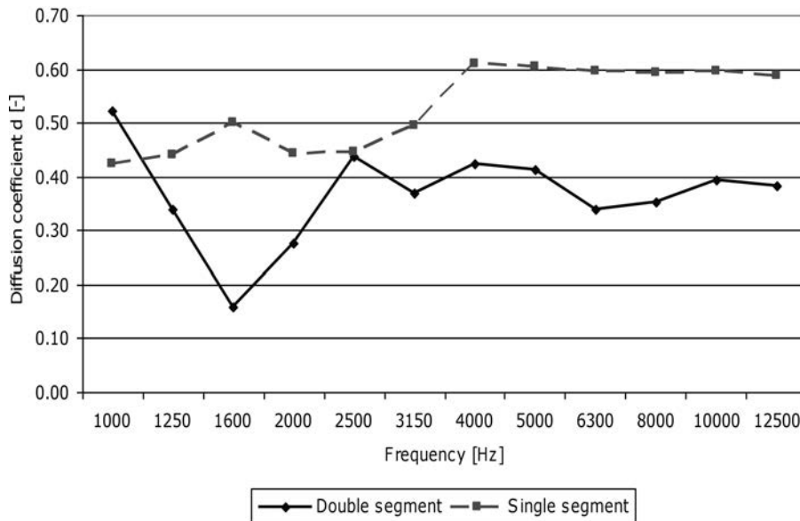
Fig. 7. Diffusion coefficient for one and two cylinder segments of the same total dimensions.
