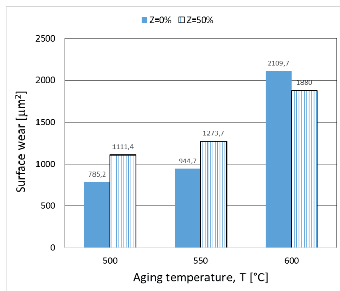
Fig. 9. Comparison of tribological wear resistance of CuTi4 alloy supersaturated and aged for 120 minutes, and supersaturated, cold worked and aged for 120 minutes
