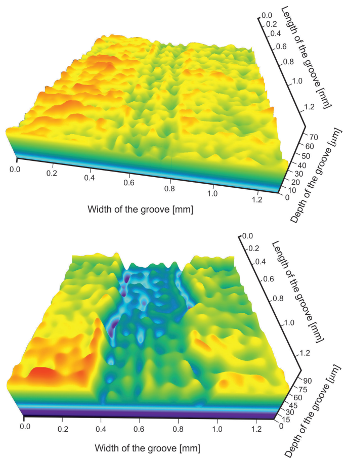
Fig. 12. Image of the scratch groove profile in CuTi4 alloy with indenter from Al 2 O 3 a) alloy supersaturated and aged next at temperature of 500°C for 120 minutes, b) alloy supersaturated, cold worked (Z=50%), and next aged at temperature of 500°C for 120 minutes, confocal microscope
