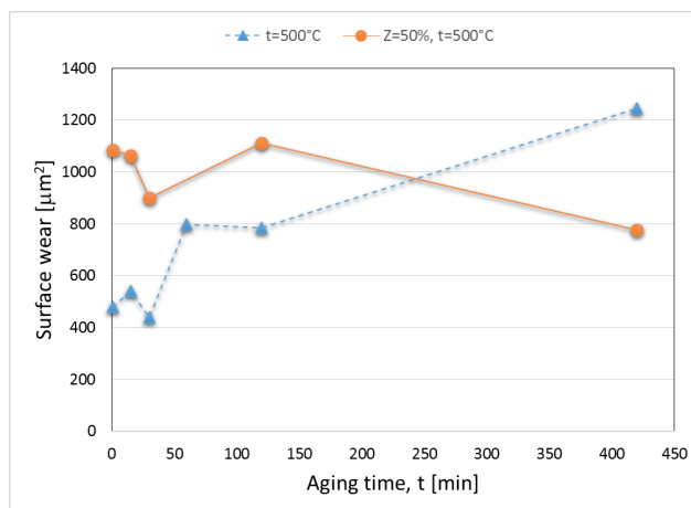
Fig. 4. Influence of ageing time at temperature of 500°C and cold rolling on abrasion wear of CuTi4 alloy supersaturated from temperature of 900°C
