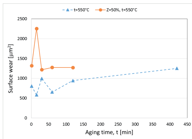
Fig. 5. Influence of ageing time at temperature of 550°C and cold rolling on abrasion wear of CuTi4 alloy supersaturated from temperature of 900°C
