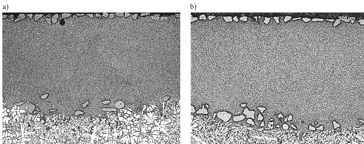
Fig. 13. Structure of the composite layer after laser surface treatment with the power: a) 1.8 and b) 2.2 kW
