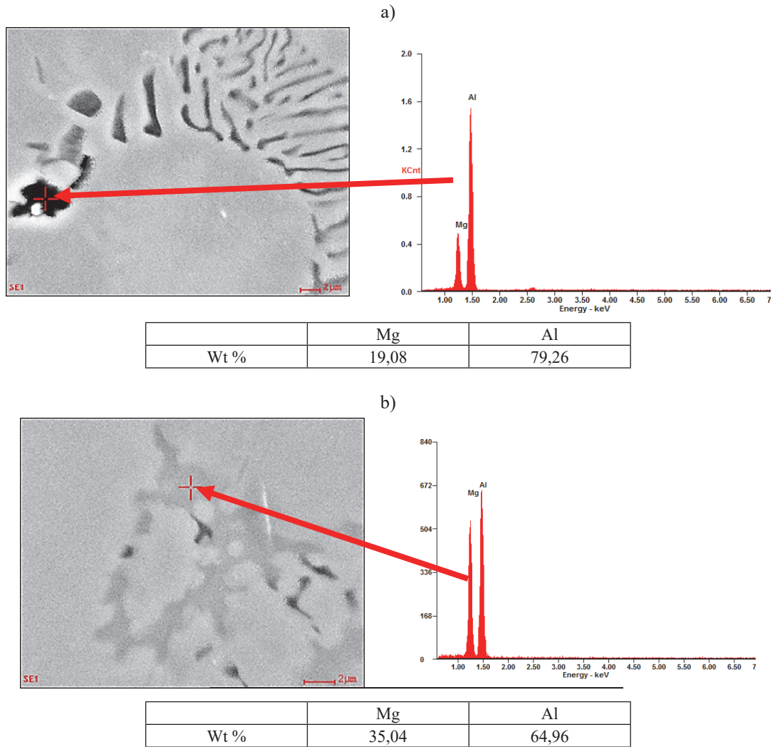
Fig 11. Analysis of chemical composition in spot of remelted area after laser treatment with the power of 2.0 kW, a) Al_4Mg b) AlMg_2
