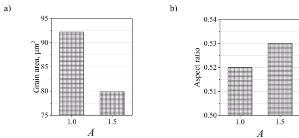
Fig. 4 Average grain size area (assuming grain boundary misorientation exceeding 5°) (a) and average aspect ratio (b) for symmetrically ( A=1.0 ) and asymmetrically ( A=1.5 ) rolled samples; thickness reduction is equal to 32%
