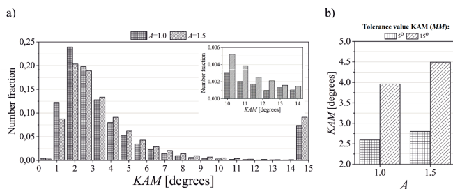
Fig. 6 Kernel average misorientation ( KAM ) distribution (a) and its average values for 5° and 15° maximum misorientations ( MM ) for symmetrically ( A=1.0 ) and asymmetrically ( A=1.5 ) rolled samples (b); thickness reduction is equal to 32%
