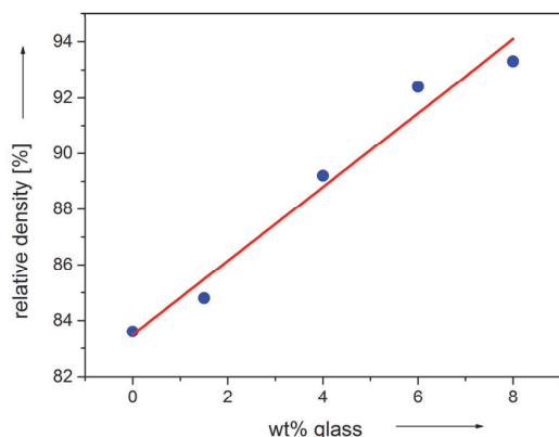
Fig. 5. The dependence of relative density of ceramics (\text{Ba}_{0.6}\text{Pb}_{0.4})\text{TiO}_3 versus the amount of glass doped
