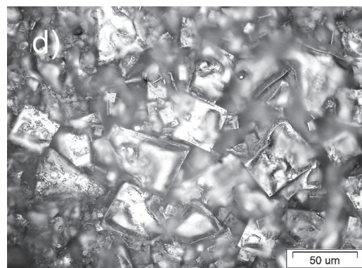
Fig. 7. The microstructure of (\text{Ba}_{0.6}\text{Pb}_{0.4})\text{TiO}_3 ceramics with different content of glass, (\text{Ba}_{0.6}\text{Pb}_{0.4})\text{TiO}_3 + 1.5 wt.% glass (a), (\text{Ba}_{0.6}\text{Pb}_{0.4})\text{TiO}_3 + 4.0 wt.% glass (b), (\text{Ba}_{0.6}\text{Pb}_{0.4})\text{TiO}_3 + 6.0 wt.% glass (c) and (\text{Ba}_{0.6}\text{Pb}_{0.4})\text{TiO}_3 + 8.0 wt.% glass (d)
