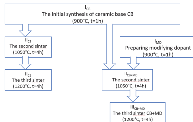
Fig. 2. Scheme of manufacturing technology of (\text{Ba}_{0.6}\text{Pb}_{0.4})\text{TiO}_3 ceramics modified with special glass
