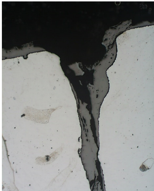
Fig. 11. A material of a welded joint (bottom generatrix – the root of the weld). A visible thermal shock crack with a distinctive wedge shape with the rest of the corrosion products. Unetched metallographic specimen. Zoom 50×
