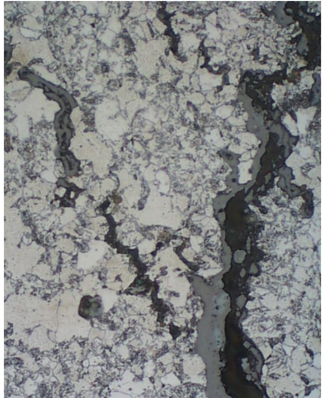
Fig. 8. HAZ – the bainite type of a structure. The disintegration of the primary structure, grids of intercrystalline macro and microcracks, and the chains of creeping micropores on the grain boundaries. Zoom 500×
