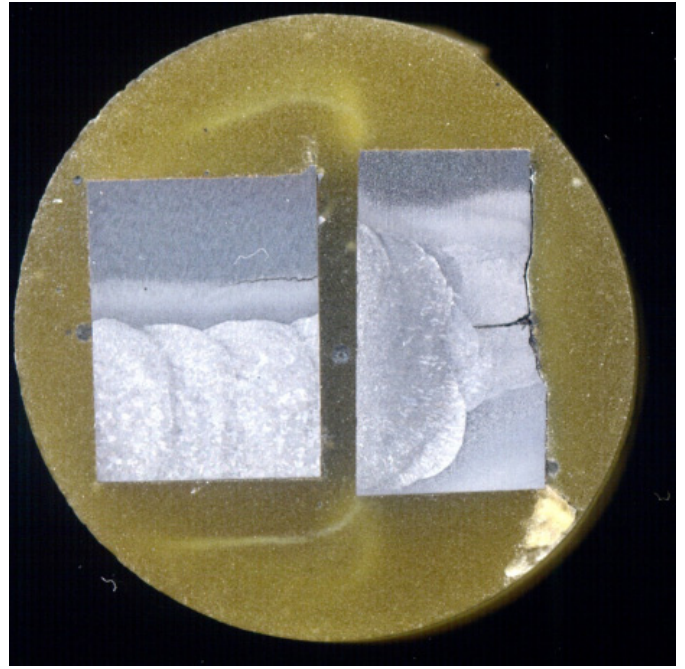
Fig. 5. The view from the face of the weld, an outer surface – a crack in the HAZ and a cross section – a crack in the weld from the root side of the weld
