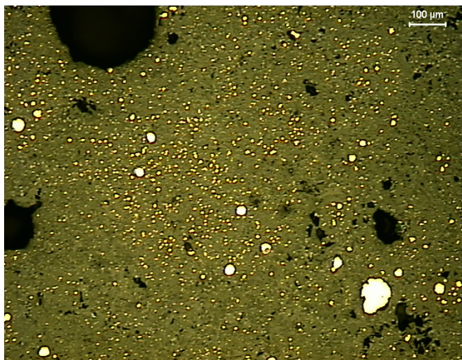
Fig. 4e. Post-processing slag containing the copper droplets; as treated by the CaO, NaCl, and Na 2 CO 3 – chemicals in the conditions similar to those usually applied to the industrial practice
