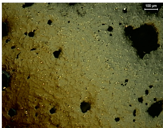
Fig. 1. Copper droplets / liquid slag suspension; a/ with the partial agglomeration of the copper droplets as caused by the addition of the CaO – chemical in the electric arc furnace in the Smelter and Refinery Plant, Głogów, b/ with an essential agglomeration and coagulation of copper droplets as caused by the addition of the NaCl, CaO, CaC 2 , Na 2 CO 3 – chemicals (and others, [3]).
