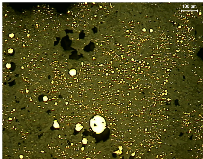
Fig. 4f. Post-processing slag containing the copper droplets; as treated by the CaO, CaC 2 , NaCl, and Na 2 CO 3 – chemicals in the conditions similar to those usually applied to the industrial practice
