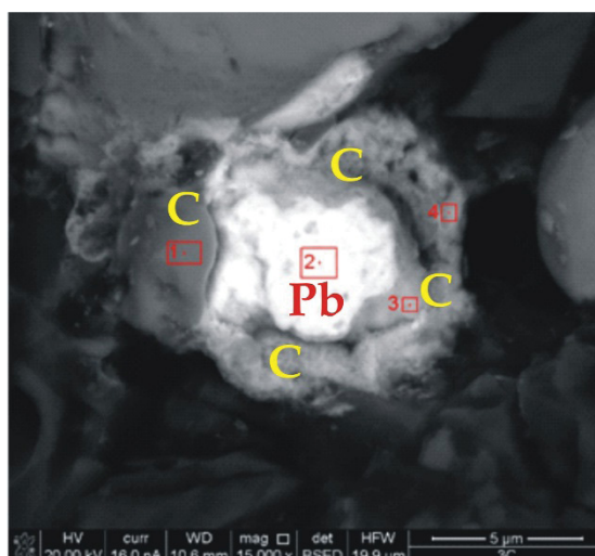
Fig. 3c. Separation of the lead droplet by carbon's envelope
