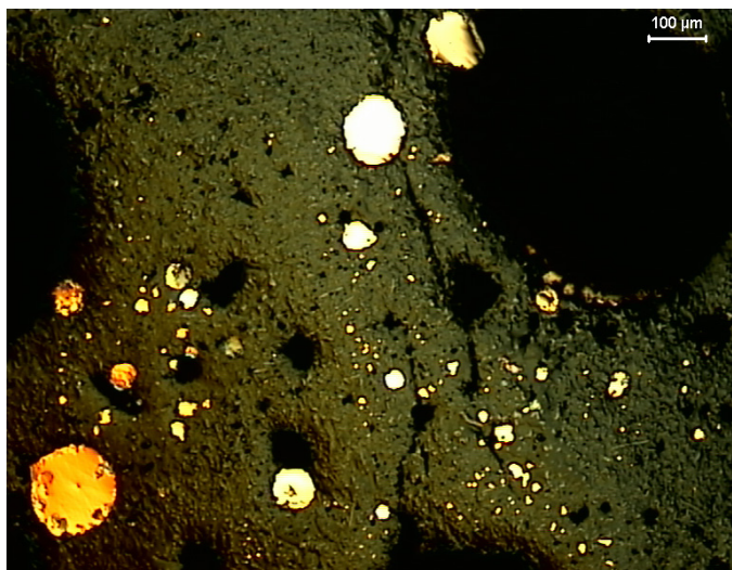
Fig. 4g. Post-processing slag containing the copper droplets; as treated by the CaO, CaC 2 , NaCl, K 3 PO 4 , and Na 2 CO 3 – chemicals (and others, [3]) in the conditions similar to those usually applied to the industrial practice
