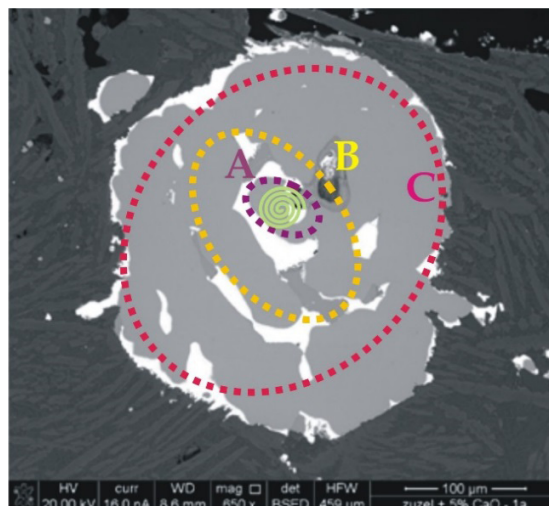
Fig. 3g. Triple droplet; every component droplet: A, B, and C, is accompanied by its individual lead envelope, just before formation of the final / general lead envelope; three copper droplets are in course of the rotation (green spiral) and coagulation; unfortunately, the final / general lead envelope will block further coagulation
