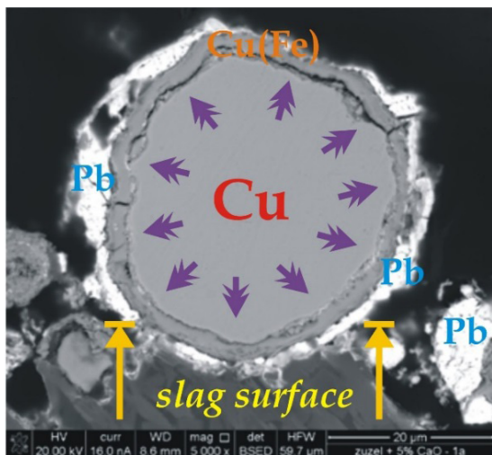
Fig. 3f. Self-cleaning of the copper droplets due to centrifugal force which appears as a result of the droplets rotation in the liquid slag; however, the fully cleaned copper droplet is surrounded by: Cu(Fe), and Pb – envelopes which block the further coagulation of the droplet; buoyancy force pushed the droplet to the liquid slag surface (no sedimentation is possible)
