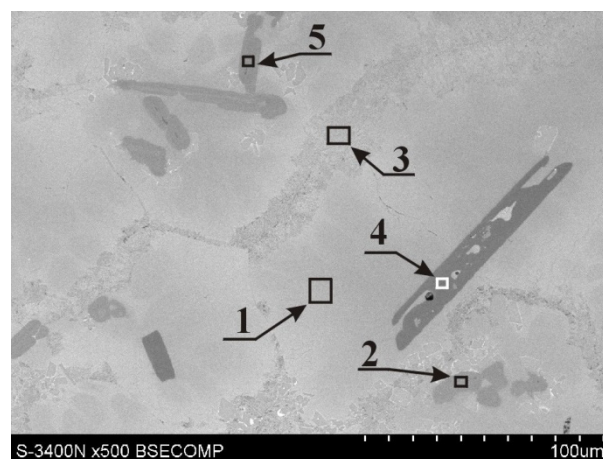
Fig. 3. As-cast microstructure of ZnAl40Cu1.5Ti1.5 alloy
