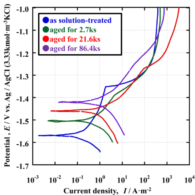
Fig. 3. Anodic polarization curves of AZ91 magnesium alloys measured in 1.029 mass% NaCl solution at 298 K
