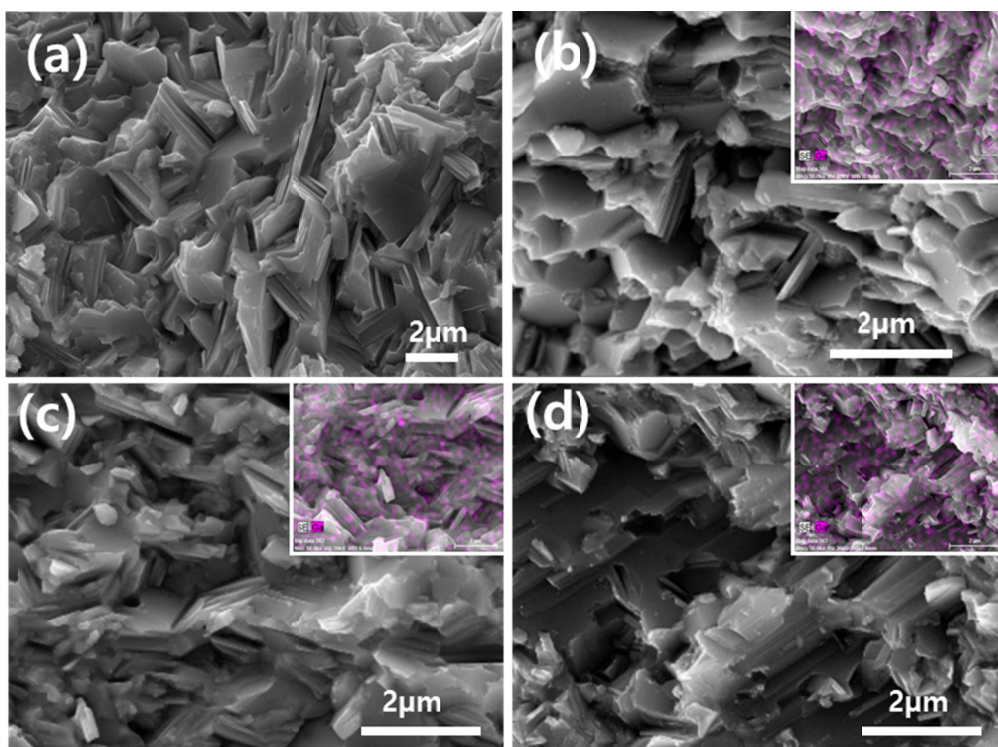
Fig. 2. Fracture surfaces of p-type \text{Bi}_{0.5}\text{Sb}_{1.5}\text{Te}_3 with (a) 0 wt% \text{Ga}_2\text{O}_3 , (b) 2 wt% \text{Ga}_2\text{O}_3 (c) 4 wt% \text{Ga}_2\text{O}_3 ,and (d) 6 wt% \text{Ga}_2\text{O}_3 bulks. The inset in (b), (c) and (d) shows the corresponding EDS mapping images
