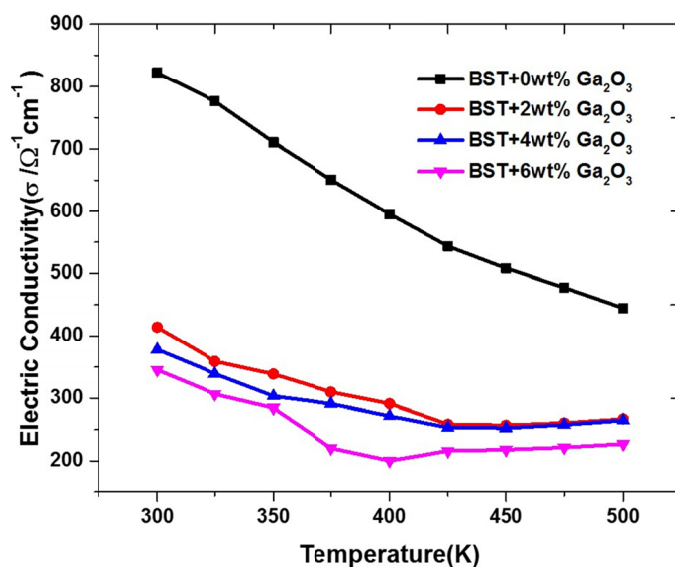
Fig. 5. Temperature dependence of electrical conductivity for \text{Bi}_{0.5}\text{Sb}_{1.5}\text{Te}_3/(x\text{-wt}\%) \text{Ga}_2\text{O}_3 ( x = 0, 2, 4 and 6\text{wt}\% ) nanocomposite bulk samples
