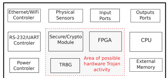
Fig. 1. Modern embedded systems as PCBs
