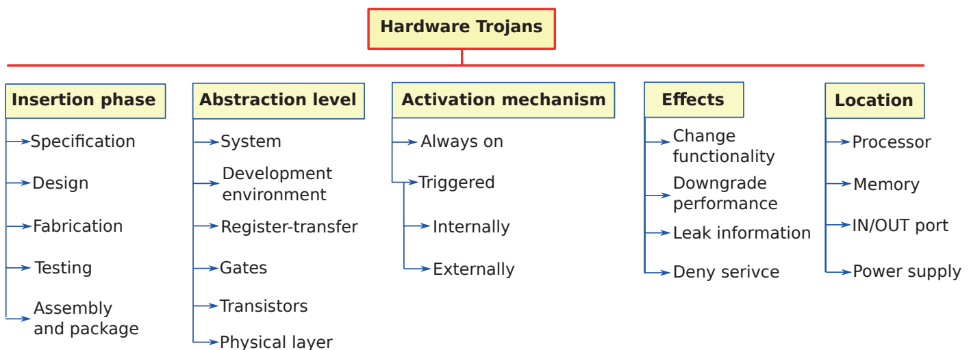
Fig. 2. Classification of the currently known HTs [11]
