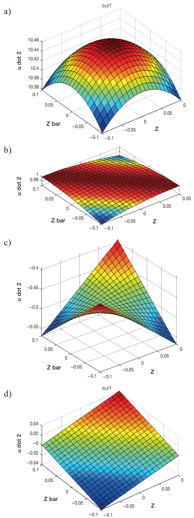
Fig. 4. a – Nonlinear changes of \dot{u}_2 with respect to \bar{z}, z for \rho(z) = z \cos(z) , b – Nonlinear behavior of \dot{u}_2 with respect to \bar{z}, z for \rho(z) = z^2 , c – Nonlinear changes of \dot{u}_2 with respect to \bar{z}, z for \rho(z) = z^4 , d – Nonlinear changes of \dot{u}_2 with respect to \bar{z}, z for \rho(z) = \sin(z)
