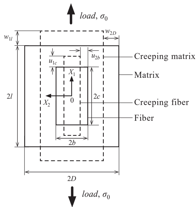
Fig. 2. Graphical explanation of the creeping fiber and matrix under tensile stress (load) “ \sigma_0 ” in X_1 -direction
