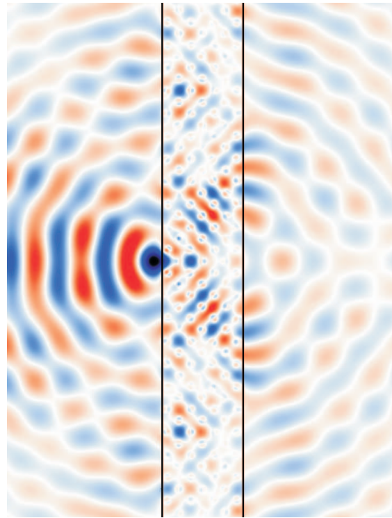
Fig. 6. Negative refraction and lensing in a cubic 3D polaritonic, dipole-like crystal
