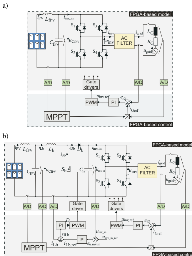
Fig. 4. The analyzed models of single-phase grid-connected systems; a) without and b) with boost converter
