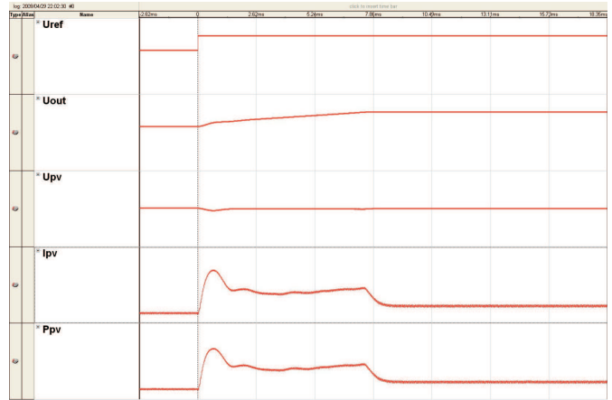
Fig. 18. Results of FPGA-based simulation of the dc-dc boost converter under closed-loop control system operation (dynamic state) – response on 300 to 400 V step of reference voltage level: U_{ref} , output voltage, PV voltage, PV current, PV power. Component values: C_{IN} = 120 \mu\text{F} , C_{OUT} = 120 \mu\text{F} , L = 720 \mu\text{H} , R = 350 \Omega . Current controller: K_P = 0.1 , T_I = 5 \text{ ms} , Voltage controller: K_P = 15 . Boost converter operating frequency: f = 18 \text{ kHz} , irradiance 1000 \text{ W/m}^2 , T = 25^\circ\text{C} . Results from QuartusII/SignalTap Logic Analyzer software
