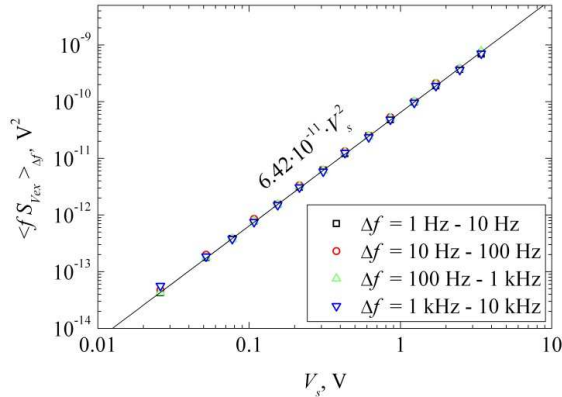
Fig. 4. The noise intensity, \langle fS_{Vex} \rangle_{\Delta f} , vs. sample voltage, V_s , for a PTFR specimen calculated for different frequency bands (points). The approximating line has a slope of 2. The measurements were carried out at room temperature.
