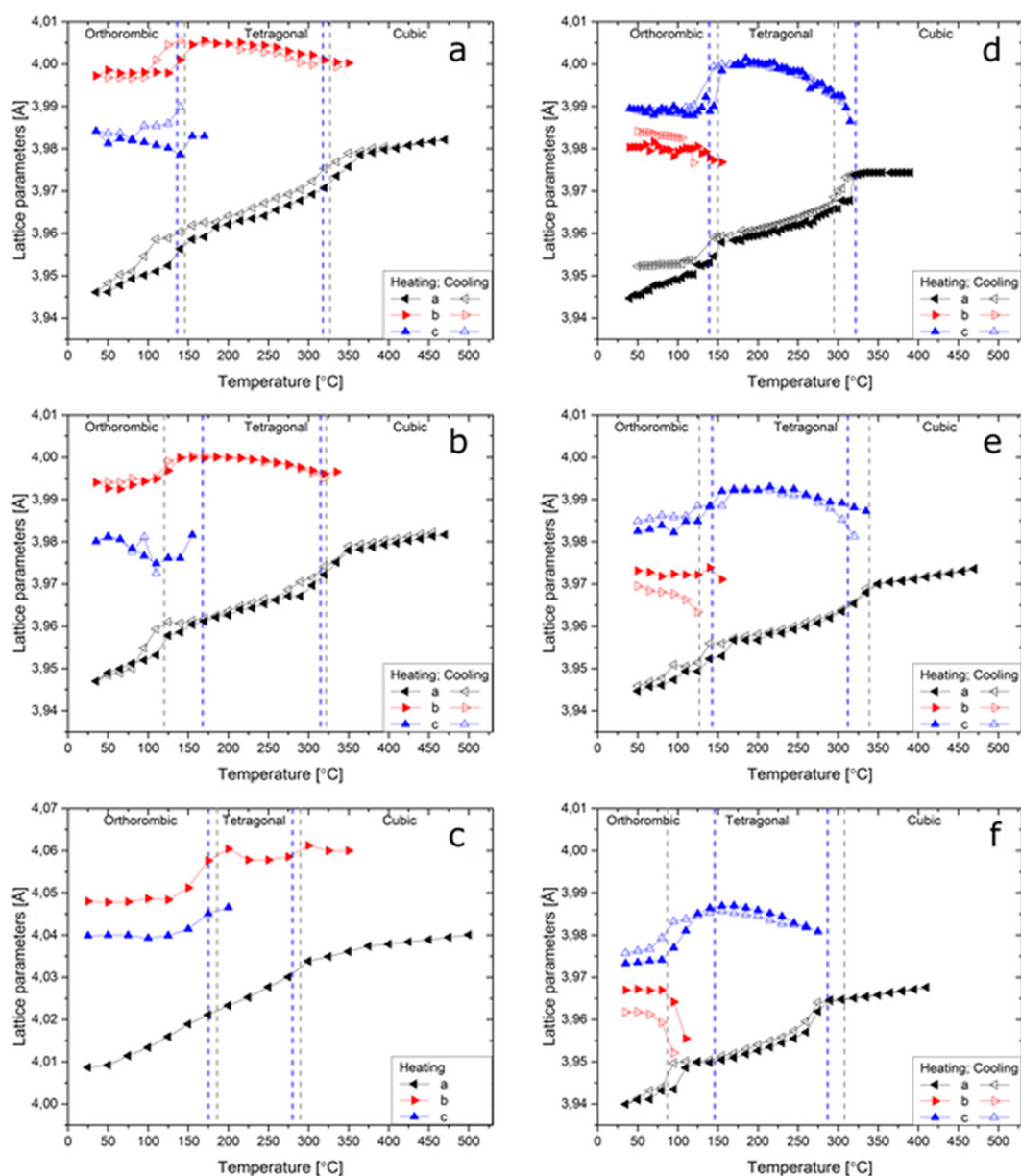
Fig. 2. Temperature dependence of lattice parameters of the Na 0.5 K 0.5 Nb 1-x Sb x O 3 (x = 0.04 (a), x = 0.05 (b) and x = 0.06 (c)) and Na 0.5 K 0.5 Nb 1-x Sb x O 3 + 0.5 mol% MnO 2 (x = 0.04 (d), x = 0.05 (e) and x = 0.06 (f)) ceramics during heating (filled symbols) and cooling (empty symbols) cycles determined from the X-ray diffraction measurements. Vertical lines correspond to the phase transition temperatures determined from the DSC (grey) and the dielectric (blue) measurements
