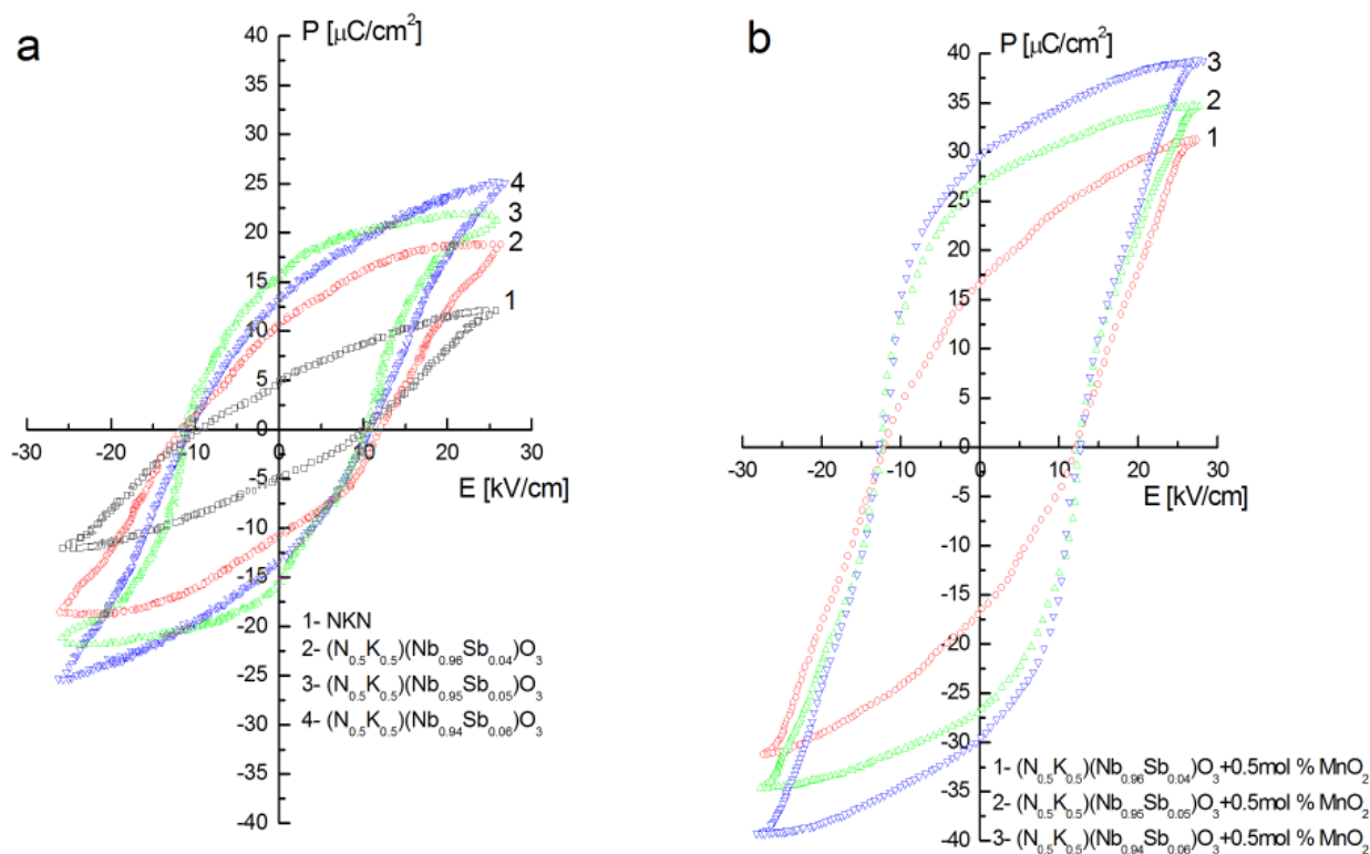
Fig. 6. Room temperature P-E hysteresis loops of the NKN and NKNS (a) and NKNS + 0.5 mol%MnO 2 (b) ceramics
