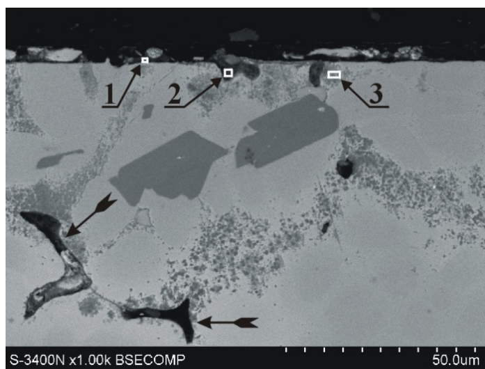
Fig. 5. Structure of surface layer of ZnAl40Ti2Cu after supersaturation and aging 385°C/24 h + 125°C/1 h after corrosion tests in „acid rain” (pits marked)
