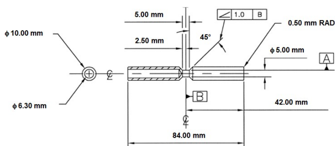
Fig. 1. Drawing of the sample for dilatometric tests
