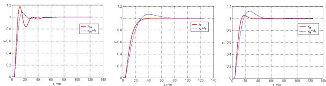
Fig. 2. The response of the control system at the step excitation for case 1
