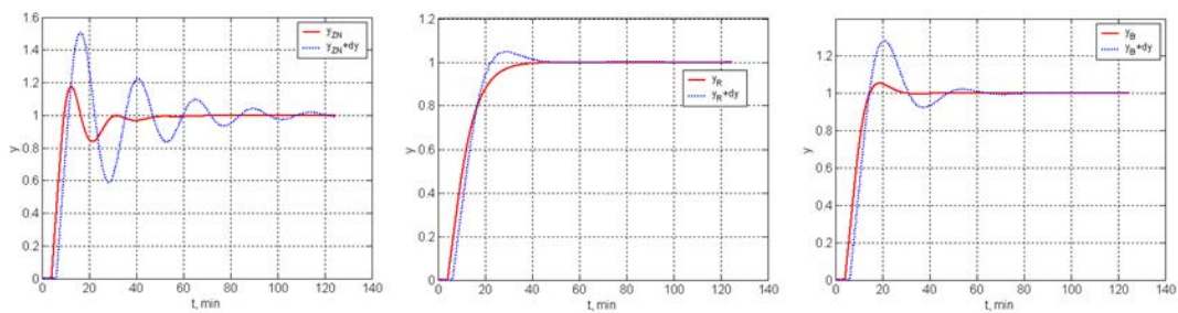
Fig. 4. The response of the control system at the step excitation for case 3
