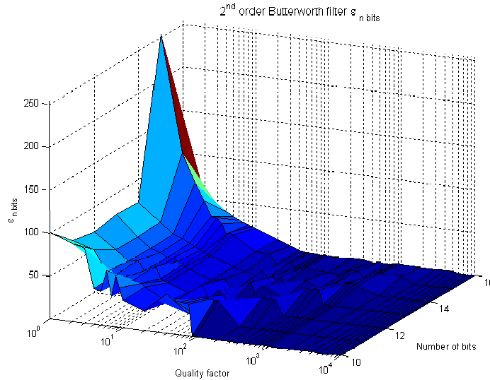
Fig. 3. Second order fixed-point Butterworth filter \epsilon_n bit. Normalized cut-off frequency of 0.05, n from 10 to 16 bits, and Q_{test} vector.
