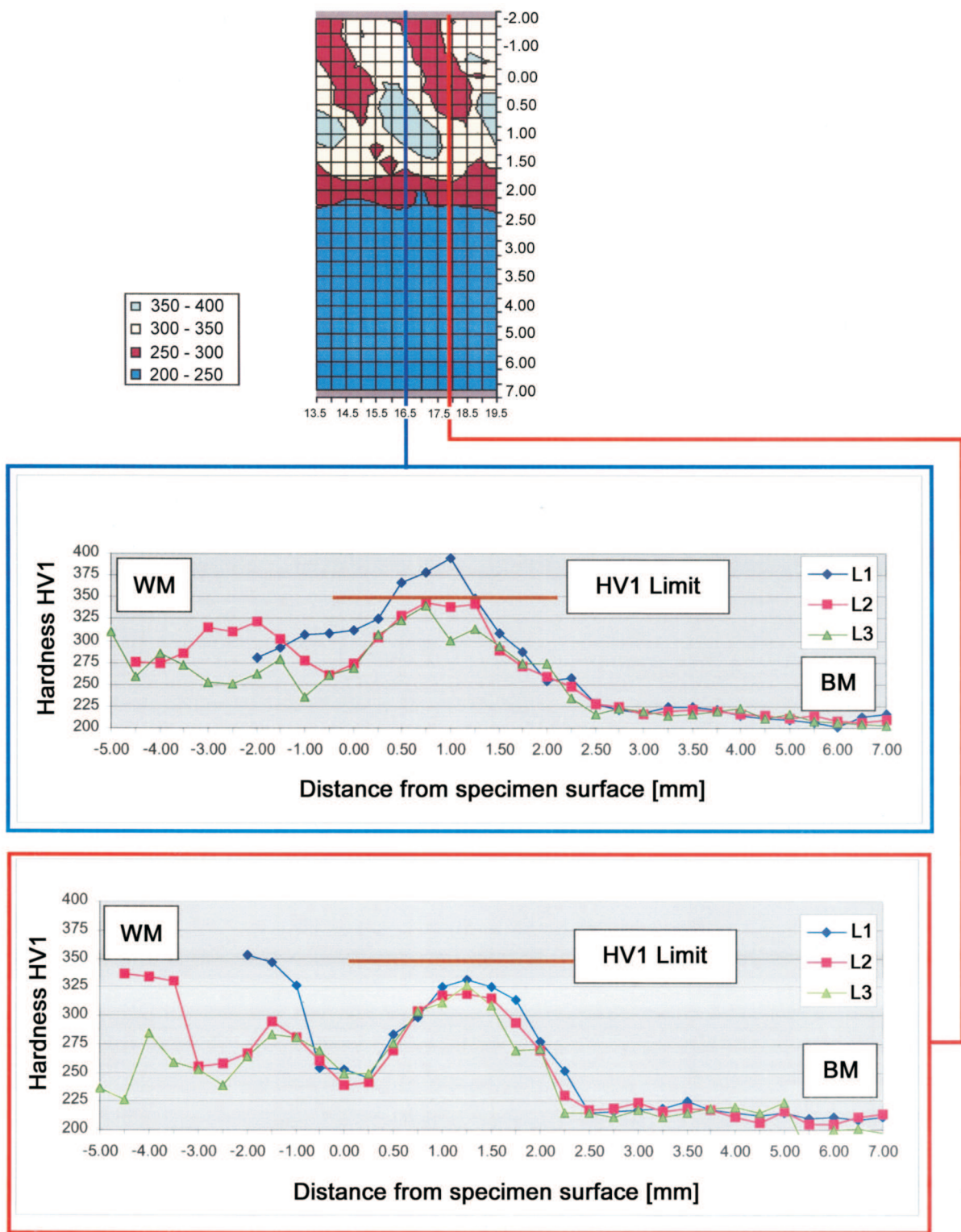
Fig. 11. Tempering Mode: Hardness HV1 measurement after manufacturing of 1 st , 2 nd and 3 rd Layer. Hardness evolution in regions, which were hardened or tempered during manufacturing of 1 st Layer [7]
