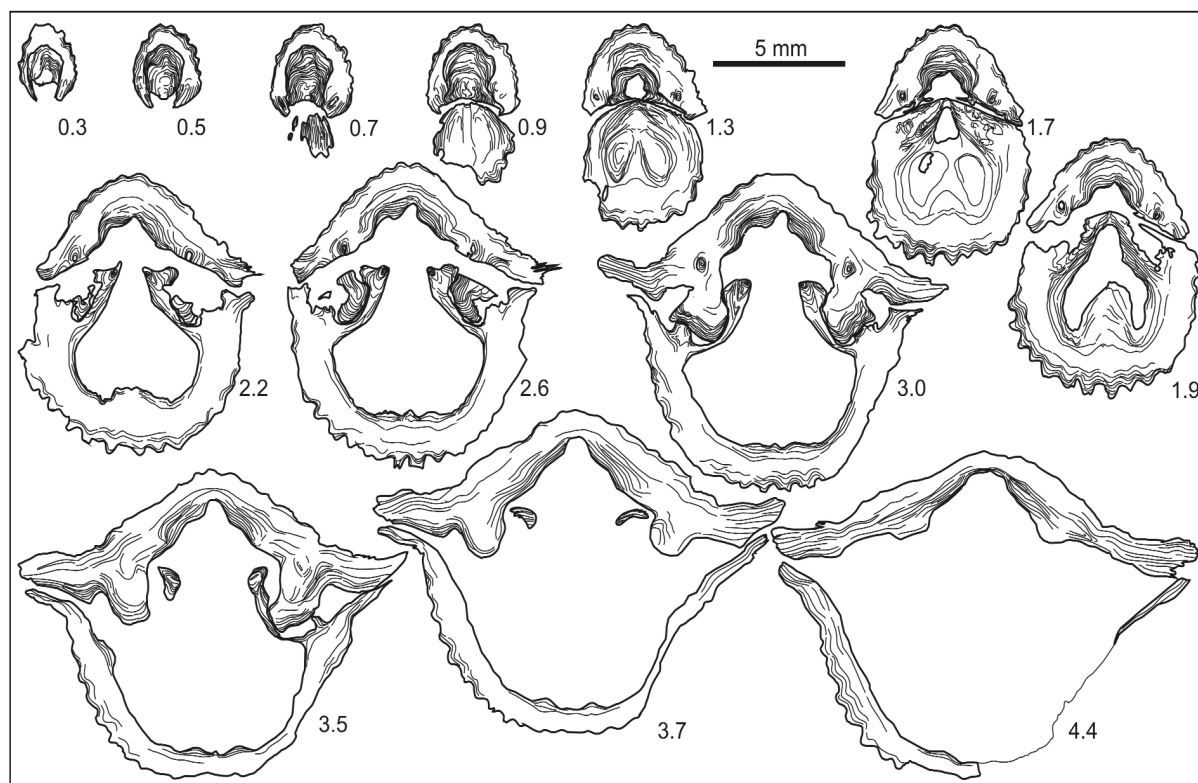
Text-fig. 11. Transverse serial sections of Atryparia ( Costatrypa ) agricolae sp. nov. through the shell ZPAL Bp 73/2/16/9 from Radlin (middle Szydlówec Beds). Numbers refer to distances in mm from ventral umbo
