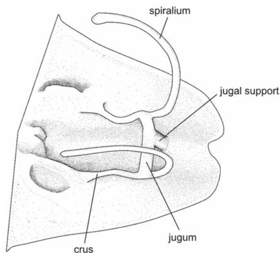
Text-fig. 15. Reconstruction of dorsal valve interior of Komiella devonica Ljaschenko, 1985 showing details of the structure of the spiraliun
