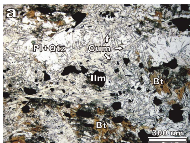
Text-fig. 13. a. Photomicrograph of cummingtonite crystals in amphibolite from the northern contact zone (the Szklarska Poręba belt); one polarizer. Abbreviations: Bt – biotite, Cum – cummingtonite, Ilm – ilmenite, Qtz – quartz, Pl – plagioclase. b. Chemical composition of cummingtonite from the northern contact zone (Szklarska Poręba belt, yellow field) and the south-eastern contact zone (Sowia Dolina, green field). Mineral data from Ilnicki (2002, 2011)
