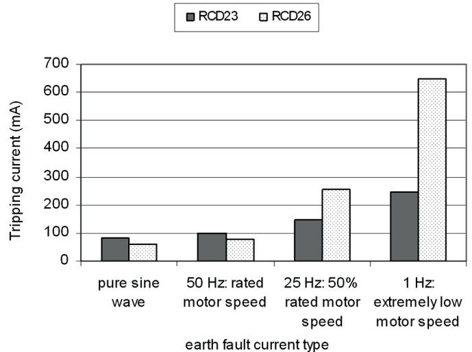
Fig. 19. Tripping current of the selected two RCDs of I_{\Delta n} = 100 mA (RCD23: AC-type; RCD26: A-type) for modelled variable-speed drive earth fault currents
