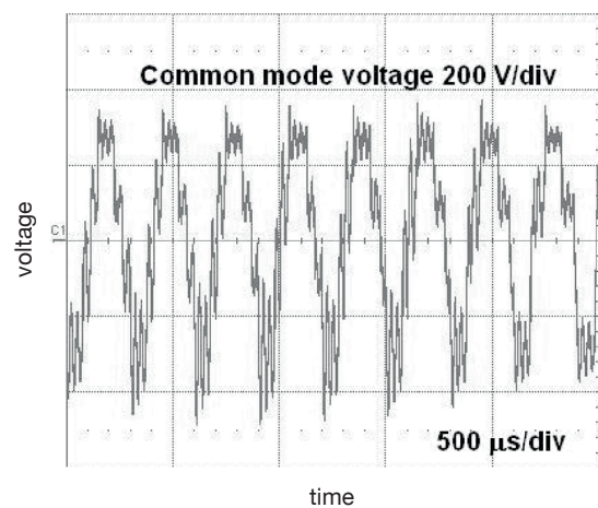
Fig. 6. The waveform of common mode voltage for LCF filter under normal operation – no earth fault, f_{1\text{har}} = 25 Hz [18]
