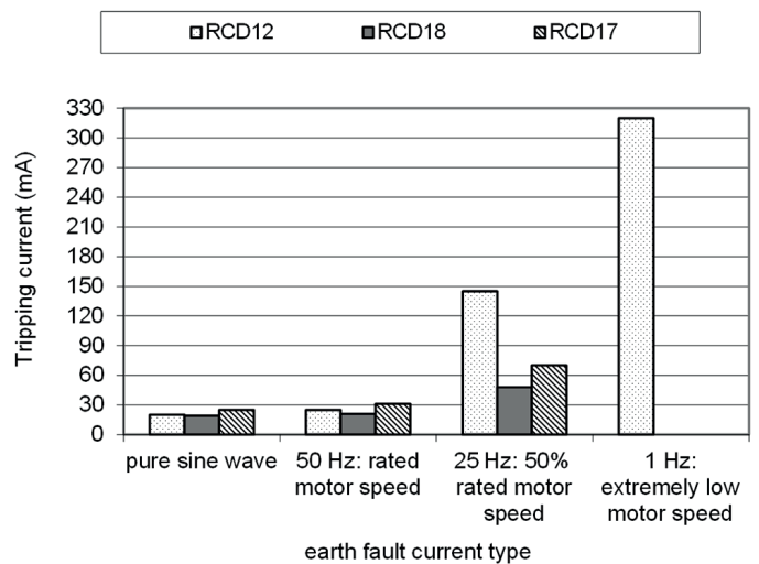
Fig. 18. Tripping current of the selected three RCDs of I_{\Delta n} = 30 mA (RCD12, RCD17, RCD18: A-type) for modelled variable-speed drive earth fault currents
