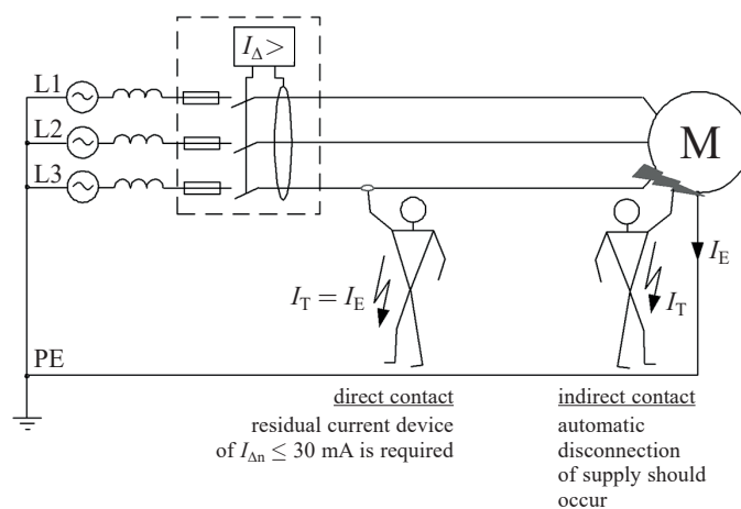
Fig. 1. Direct and indirect contact in a circuit, and requirements to achieve safety; ( I_{\Delta} > ) – residual current device, I_E – earth fault current, I_T – touch current
