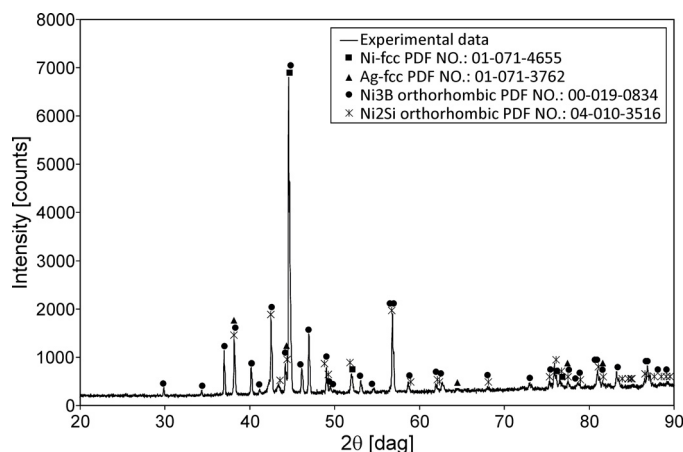
Fig. 2. X-ray diffraction pattern of the Ni-Si-B-Ag arc-melted ingot
