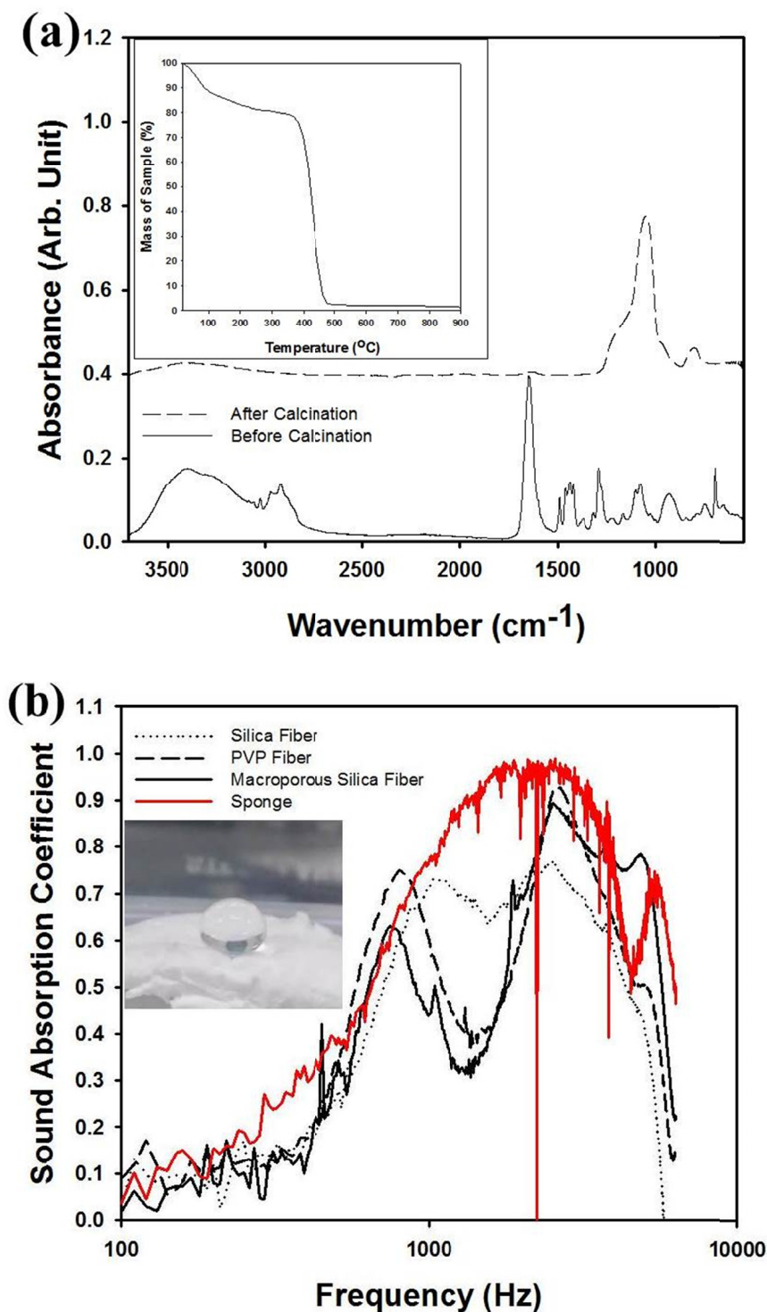
Fig. 4. (a) FT-IR analysis results of fibrous materials before and after calcination at 500^{\circ}\text{C} . The inset figure presents the TGA result of electro-spun fibers. (b) The sound absorption coefficient of PVP fibers, silica fibers without macropores, macroporous silica fibers having macropores with 700 nm in diameter, and commercial sponge as a function of the frequency of incident acoustic wave. The inset figure presents the photograph of water droplet on macroporous silica fibers having macropores with 700 nm in diameter. The fibrous materials were treated with fluorine-containing silane coupling agent
