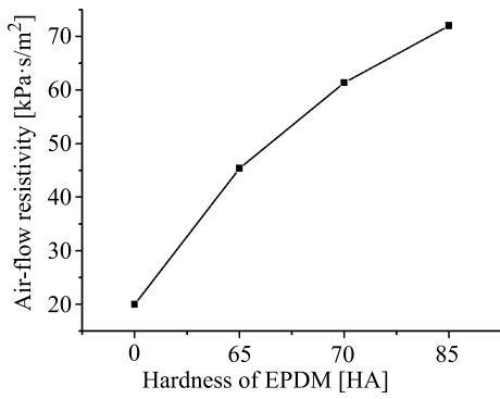
Fig. 8. Air-flow Resistivity of PU foams which filled with EPDM of different hardness.
