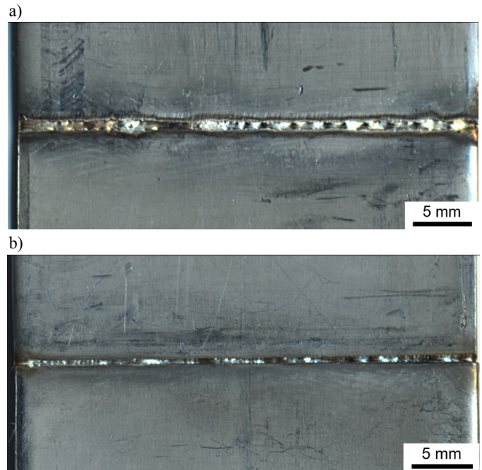
Fig. 4. A view of the butt joint of 2.0 mm sheet of AISI 304 stainless steel laser welded by the disk laser at output power 1.5 kW, welding speed 4.0 m/min, and focal spot position -1.0 mm (Table 3); a) weld face, b) root surface
