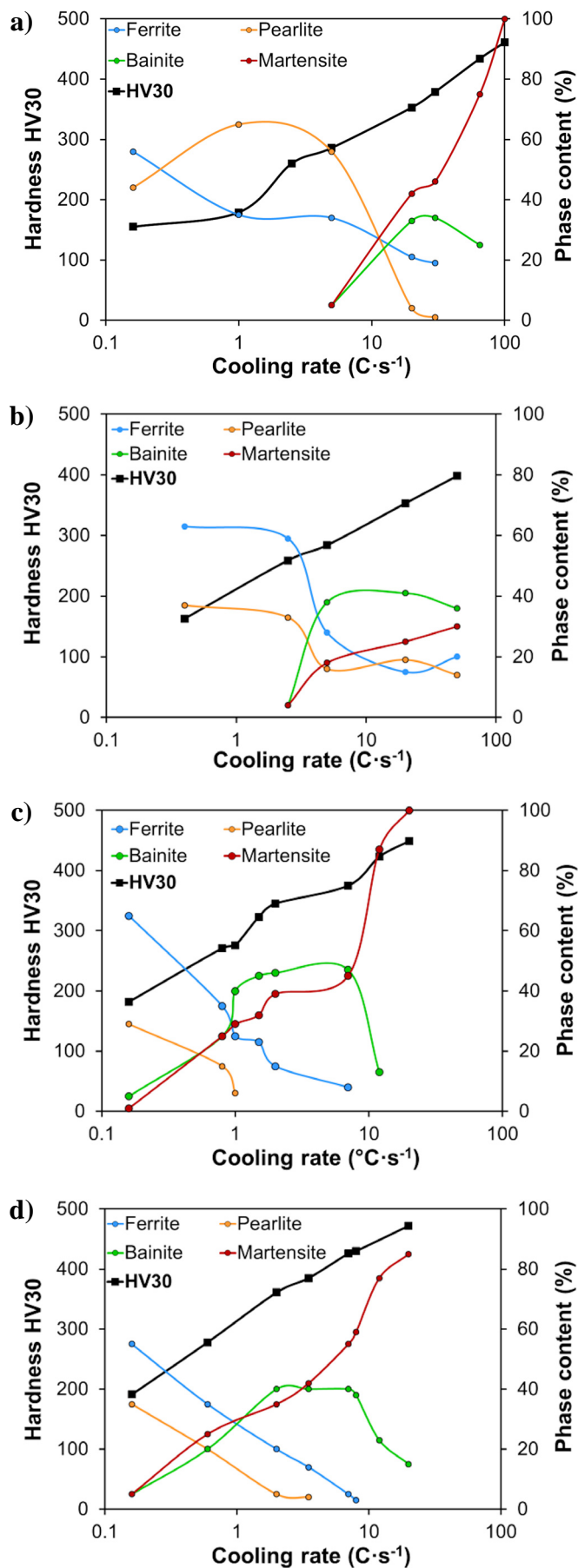
Fig. 10. a) CCT – 16MnCrS5-, b) DCCT – 16MnCrS5-, c) CCT – 20MnCrS5-, d) DCCT – 20MnCrS5 Development of structural shares and measured hardness of HV30 depending on cooling rate
