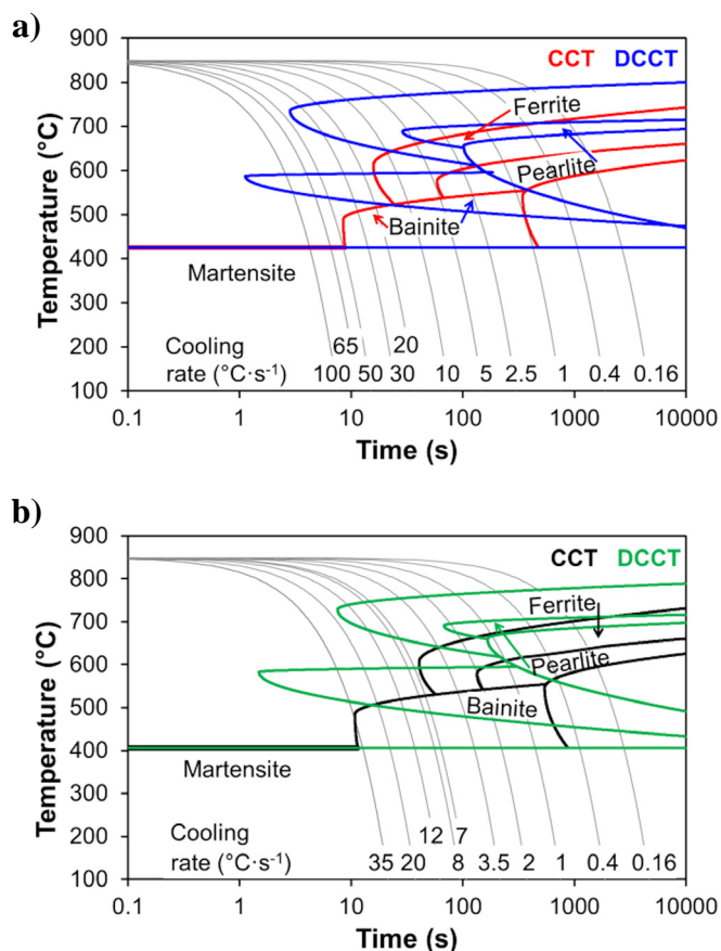
Fig. 11. a) 16MnCrS5, b) 20MnCrS5, CCT and DCCT diagrams of the steels 16MnCrS5 and 20MnCrS5 designed with help of the QTSteel 3.2. Software
