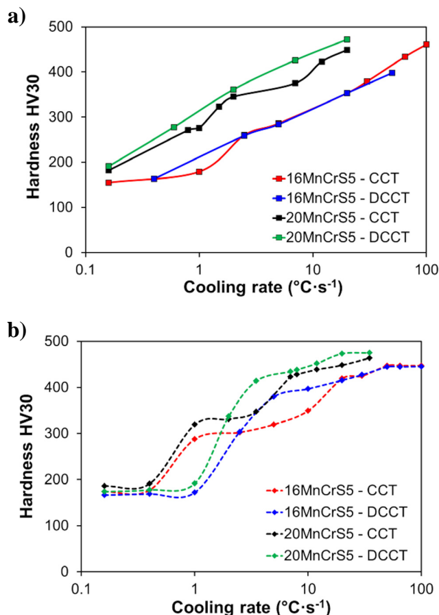
Fig. 12. a) Dilatometric tests-, b) Software QTSteel 3.2 Comparing the effect of deformation and cooling rate on hardness
