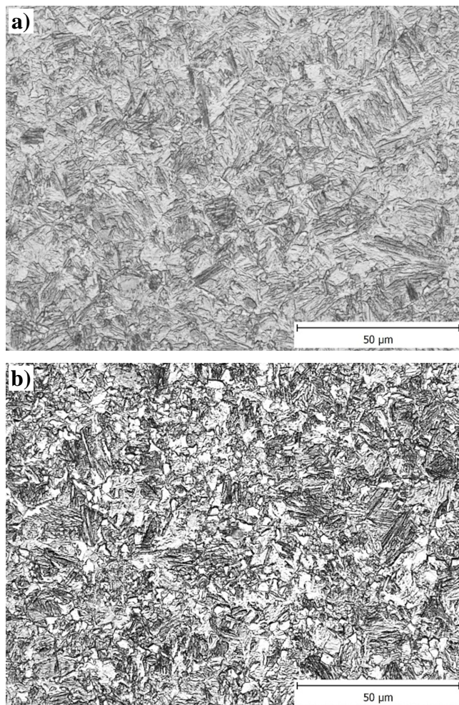
Fig. 8. a) Without deformation – cooling rate of 50°C·s -1 – 75% Martensite + 25% Bainite-, b) After deformation – cooling rate of 50°C·s -1 – 20% Ferrite + 14% Pearlite + 36% Bainite + 30% Martensite Comparison of microstructure and shares of phases of the steel 16MnCrS5 without and after deformation of selected rates
