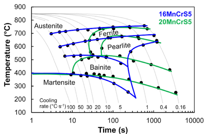
Fig. 5. Combination of DCCT diagrams of the steel 16MnCrS5 and 20MnCrS5
