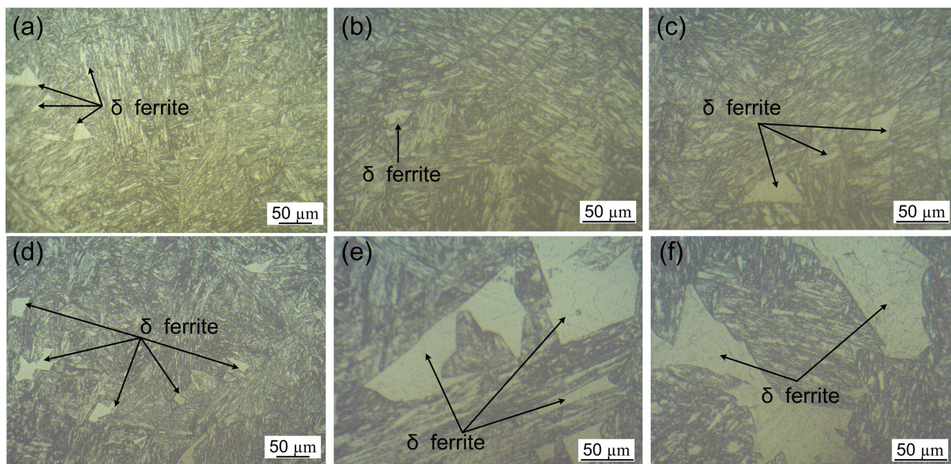
Fig. 6. Optical micrograph of the fusion zone after the PWHT for P91 steel welded joint (a), (b), and (c), respectively; fusion zone after the PWHT for P92 steel welded joint (d), (e), and (f), respectively
