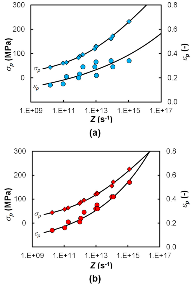
Fig. 7. Comparison of experimental values of \epsilon_p and \sigma_p (points) with predicted values (lines): (a) heating directly to the deformation temperature; (b) preheating at the temperature of 1200°C
