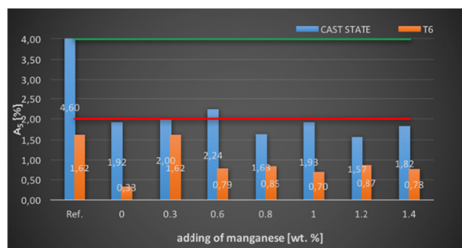
Fig. 2. Dependence of tensibility the secondary alloy AlSi7Mg0.3 with graded wt. % Mn without heat treatment and after heat treatment
