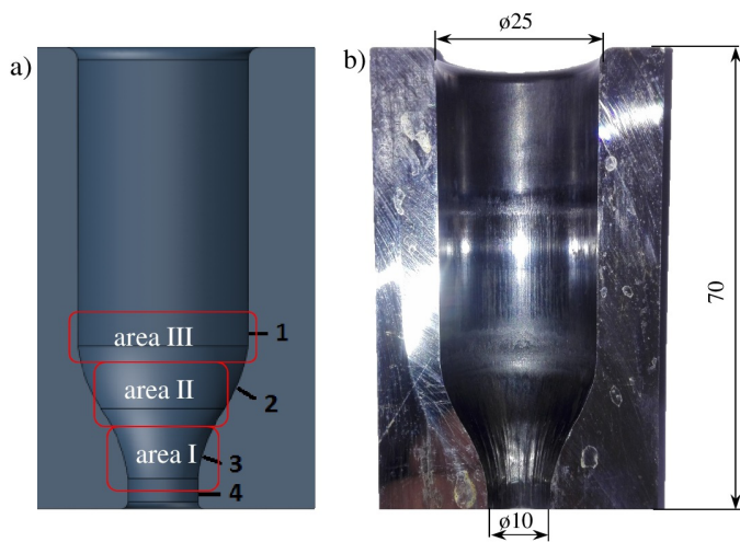
Fig. 2. View of the tool section: a) CAD model with marked selected measurement areas, including the microhardness test points, b) exemplanary image of a die's half with main dimensions in mm
