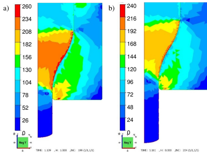
Fig. 8 Distribution of reduced stresses (von Mises): a) 1 mm to the full pocket of the punch, b) full pocket of the punch (last forging stage) in MPa
