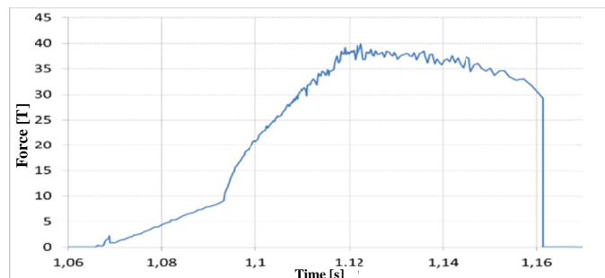
Fig. 10. Diagram of the force in I operation of extruding a valve-type element
