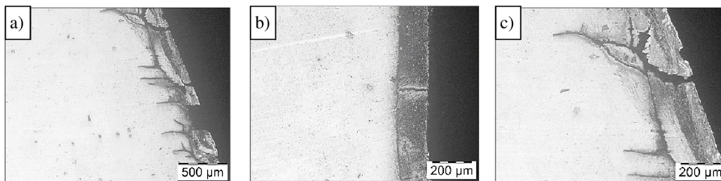
Fig. 21. Exemplary microstructural images with a visible nitrided layer and numerous cracks. The tool has produced 1900 forgings: a) in zone I, b) in zone II, c) in zone III
