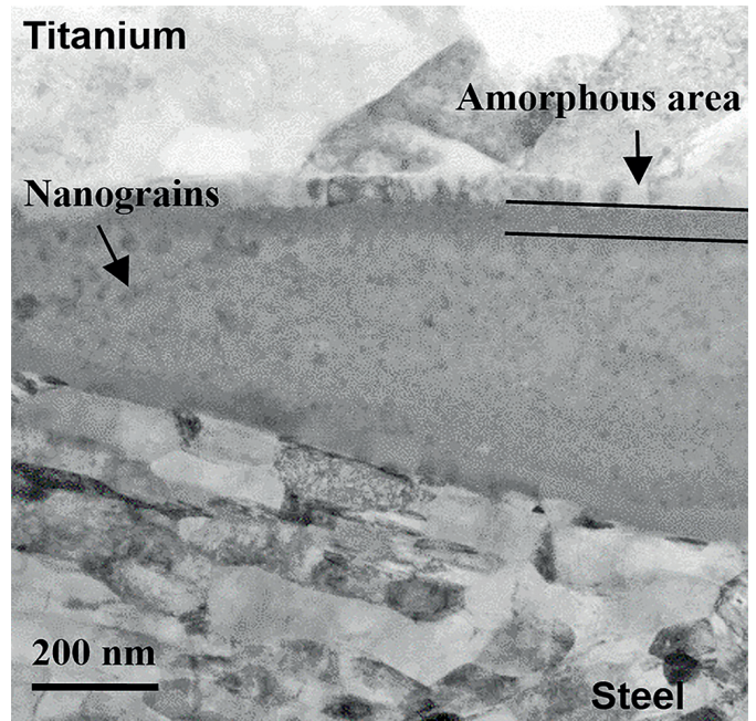
Fig. 8. Microstructure of the bond area between 316L austenitic steel and titanium prior to heat treatment
