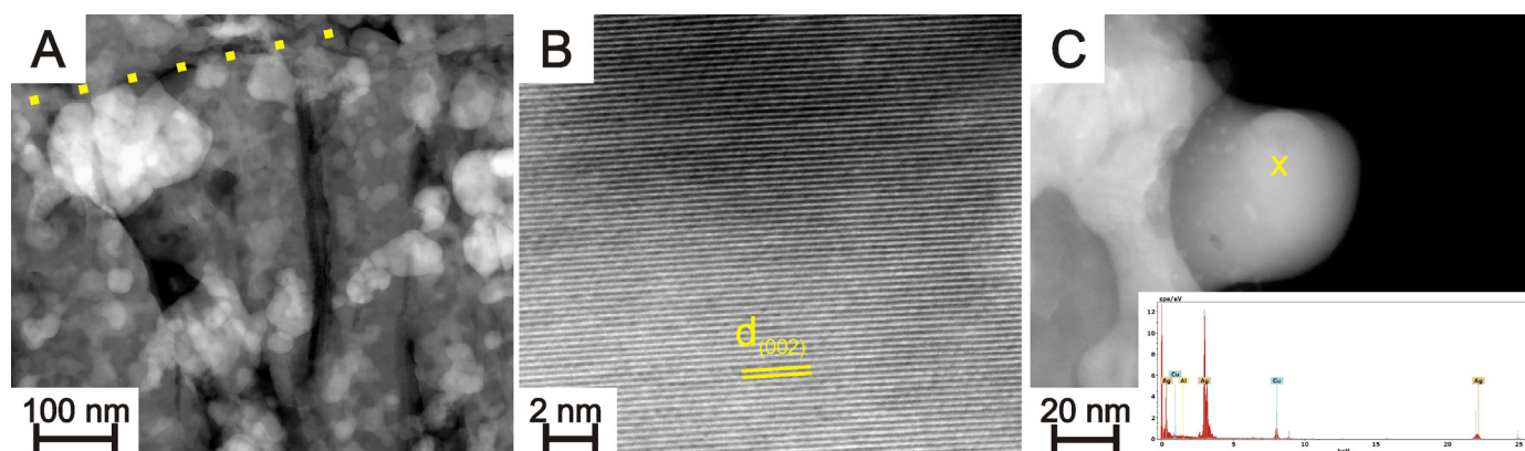
Fig. 5. HAADF-STEM images of the as-deposited Ag–Al film. Interface between tribofilm and as-deposited layer is highlighted with dot line. Inset in c) shows the EDX spectrum from the point marked with x
