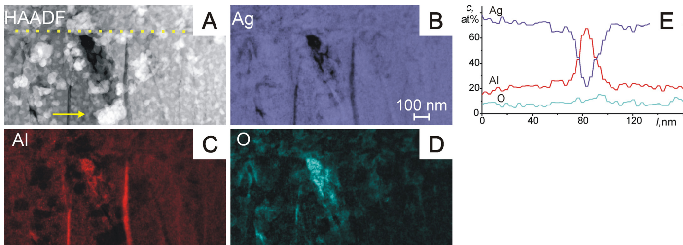
Fig. 3. HAADF image and EDX chemical element maps of the Ag–Al film. Line composition profile corresponds to the area highlighted with the arrow. Interface between tribofilm and as-deposited layer is marked with dot line
