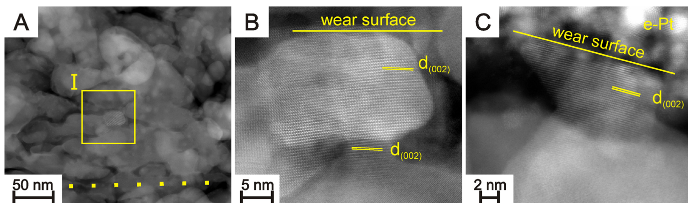
Fig. 6. HAADF-STEM images of different areas of the tribofilm. Direction of the wear surface is shown by solid line
