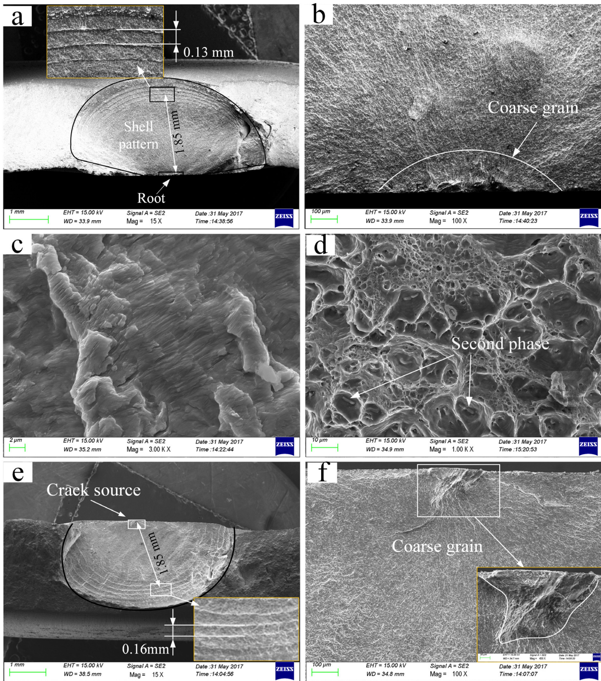
Fig. 7. Fracture morphologies: (a) specimen with stress level of 56% and its region of (b) fatigue source, (c) crack propagation, (d) final fast fracture; (e) specimen with stress level of 62% and its (f) fatigue source
