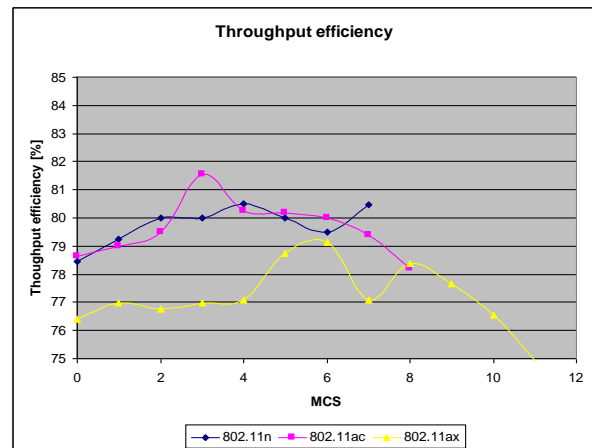
Fig. 4 Throughput efficiency
