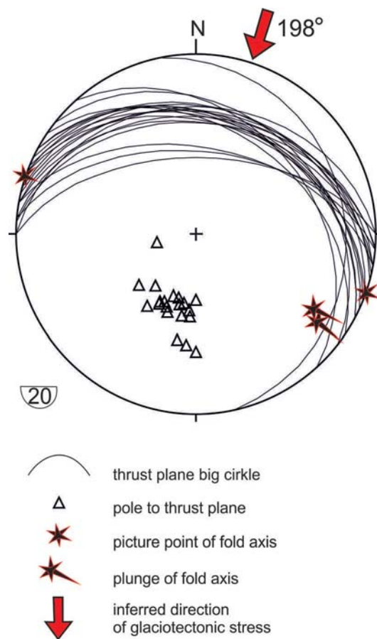
Fig. 8. Summary diagram of orientation of large-scale (first-order) glaciotectionic structures, thrust planes and fold axes, occurring in the Vistula valley scarp between Dobrzyń and Kuzki together with inferred direction of a glaciotectionic stress.
