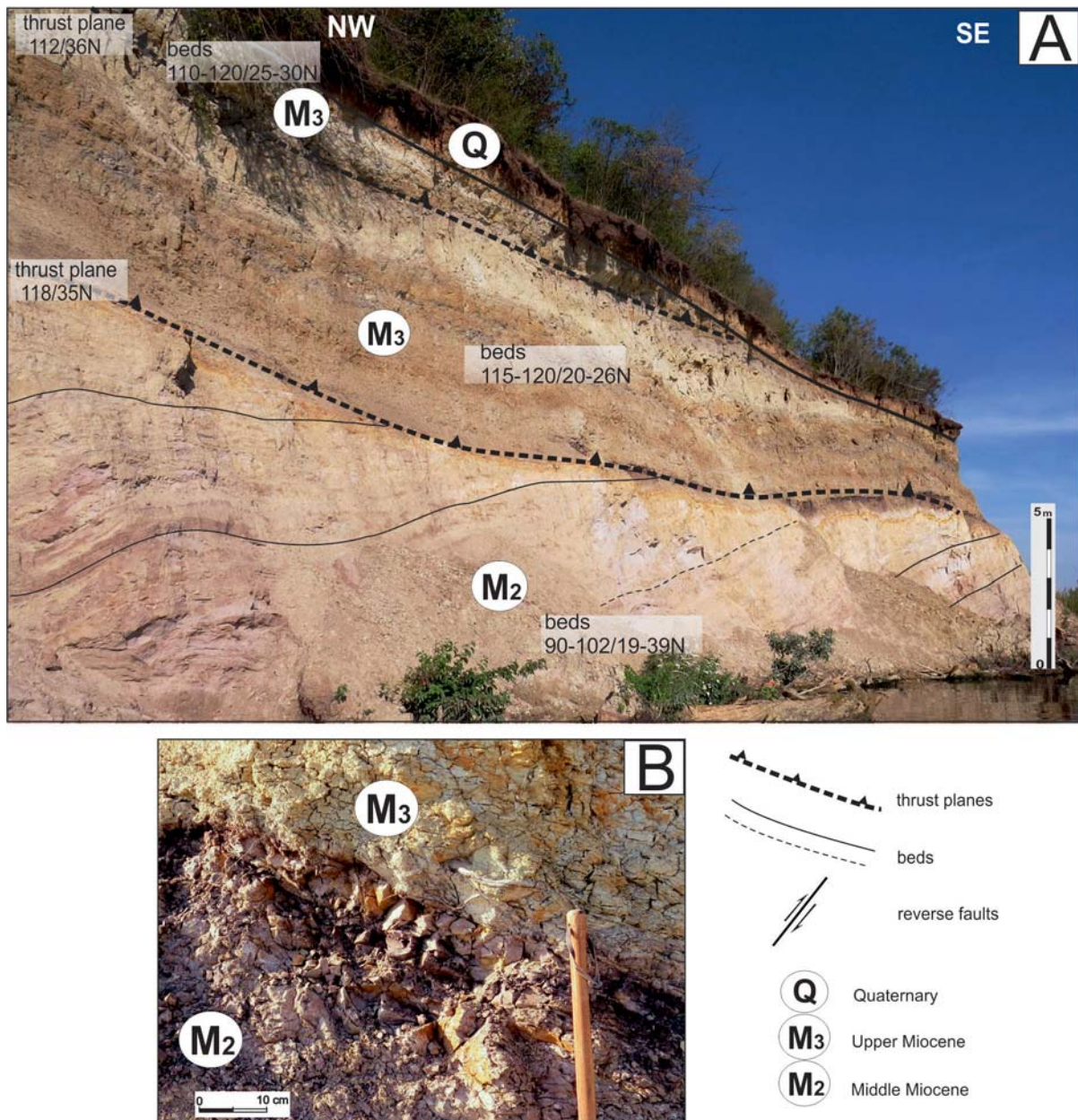
Fig. 4. The Kuzki site. A – Large-scale glaciotectionic disturbances in the Neogene deposits developed as result of thrusting from NNE. Note that both layers in particular patches and thrust planes dip to the north. B – Slip cleavage and breccia within a shear zone below the thrust sheet.
